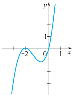
c) x_{1,2} = -2 , x_3 = 0 , p(0) = 0 ,
